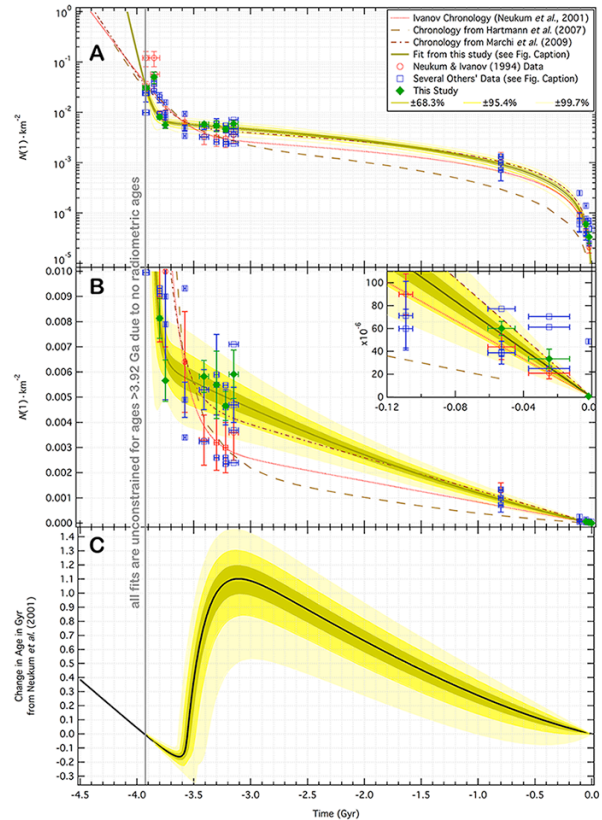
Figure 2: The canonical chronology [17] compared with revisions [13-14] and this work are in panels A and B. Panel A shows the function on semi-log axes, while Panel B focuses on the near-linear recent cratering rate on a linear plot with the last 120 Myr inset. The data points originally used by [10] and several comparison works [3-5, 8, 9-11, 14-15]. Panel C shows the difference between the new chronology and Neukum et al. [17] as a function of age in the old chronology. 1\sigma , 2\sigma , and 3\sigma confidence bands to the fit from this work are overlaid, and none of the fits are constrained for ages > 3.92 Ga.
